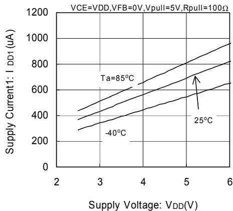
(6) Supply Current 1 vs. Supply Voltage
