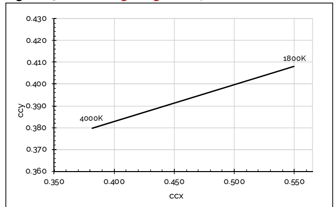
Figure 15: CCT Tuning Range, Tc=85C
