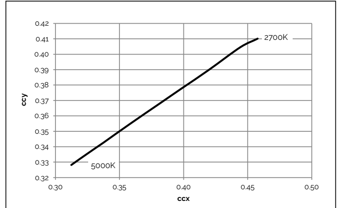
Figure 13: CCT Tuning Range, Tc=85C
