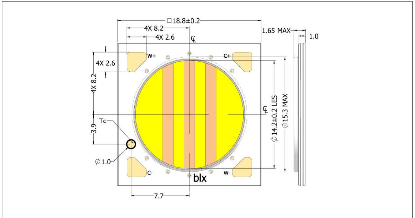
Figure 22: Drawing for Vesta Series Tunable White Gen 2 13mm Array
