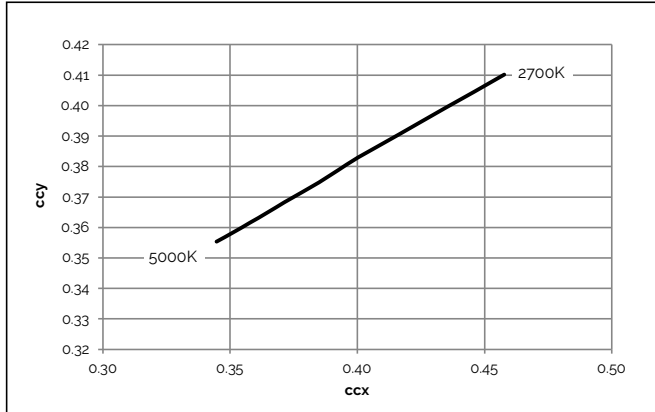
Figure 12: CCT Tuning Range, Tc=85C
