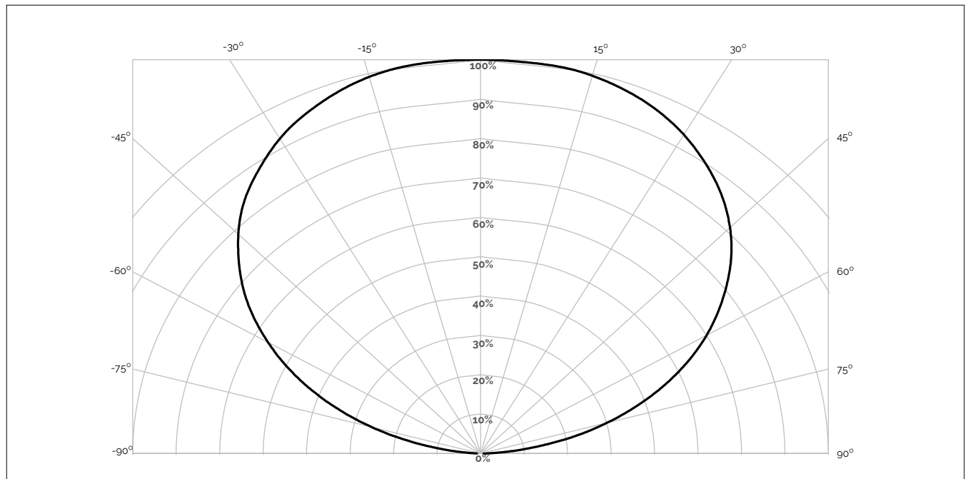
Figure 17: Typical Polar Radiation Pattern
