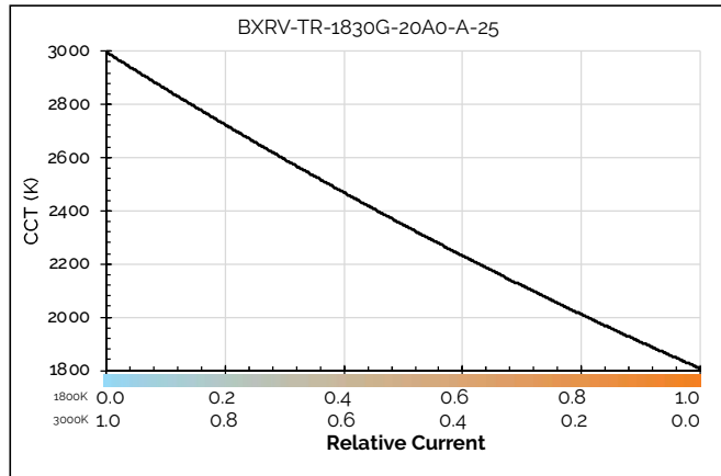
Figure 7: CCT vs. Relative Warm White Current
