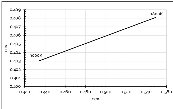
Figure 14: CCT Tuning Range, Tc=85C
