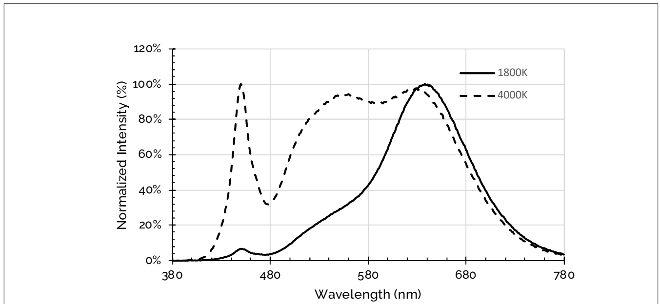
Figure 21: Typical Color Spectrum
