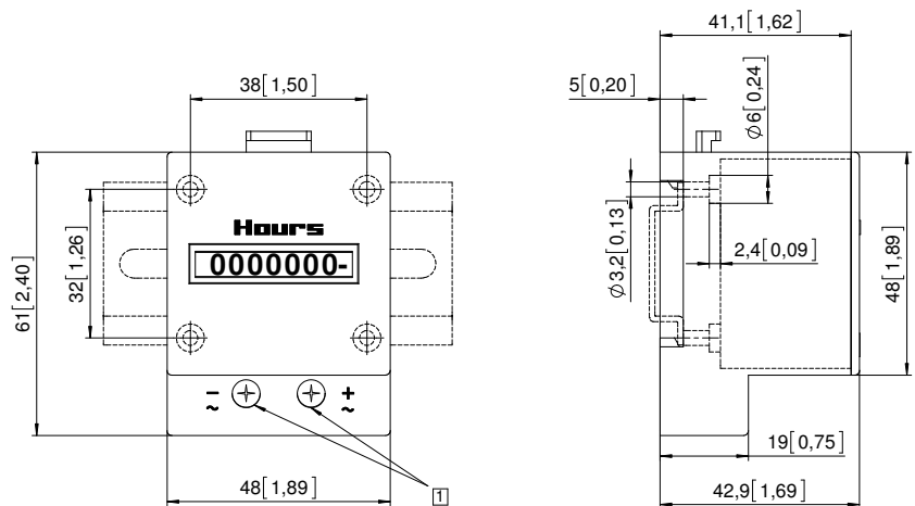
1) Screw terminals
