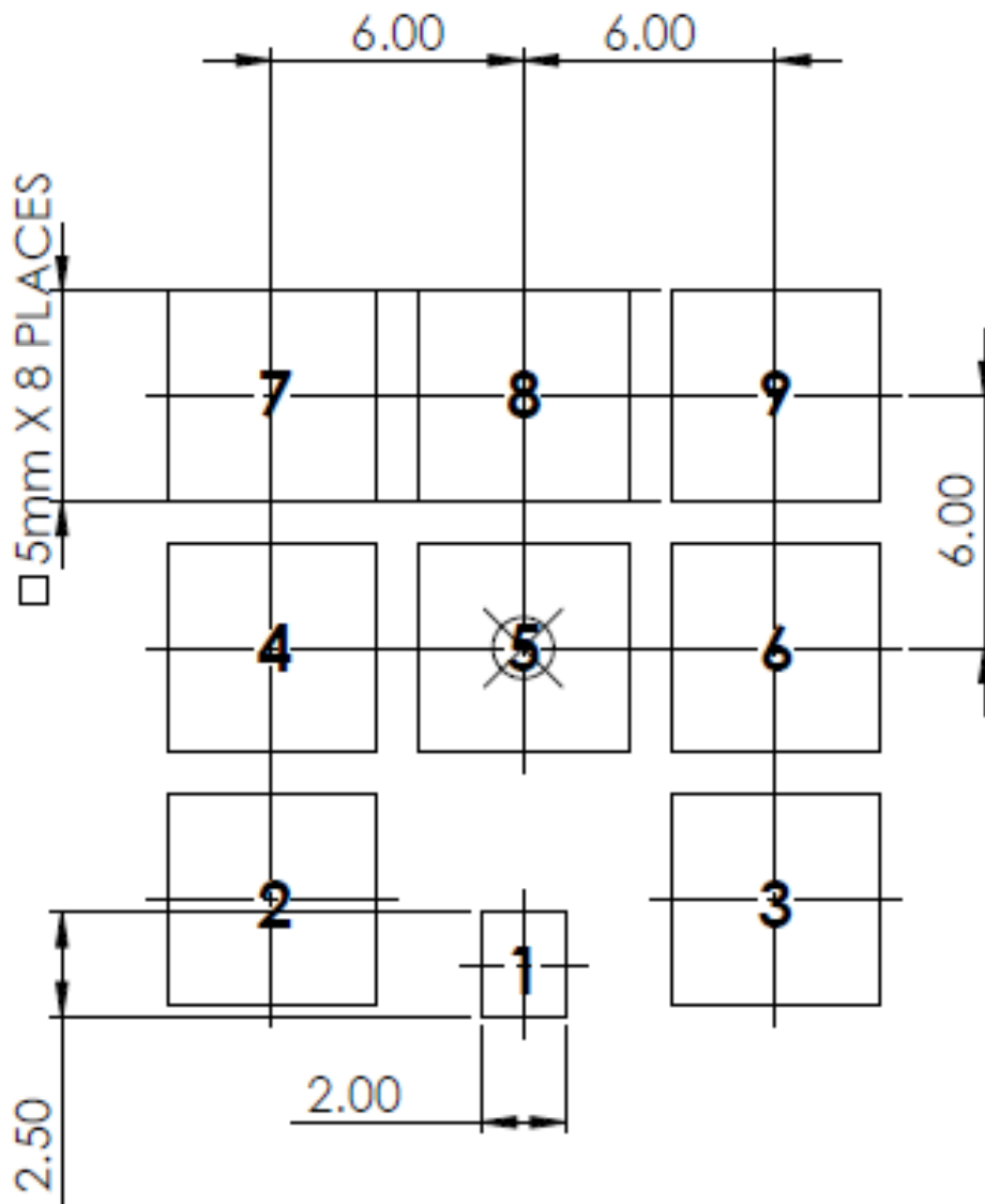
PCB FOOTPRINT
