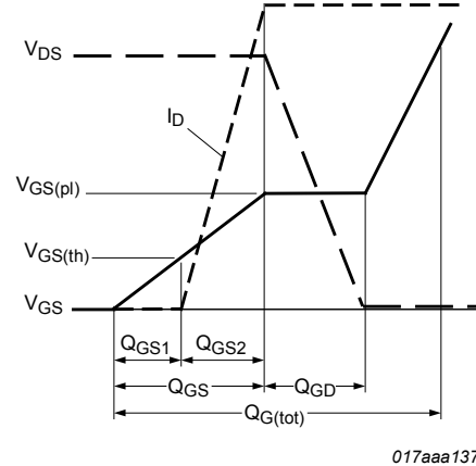
Fig. 17. MOSFET transistor: Gate charge waveform definitions
