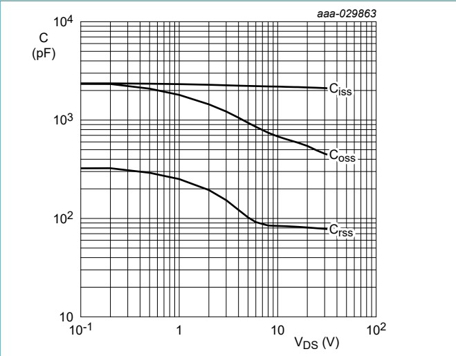
Fig. 14. Input, output and reverse transfer capacitances as a function of drain-source voltage; typical values V_{GS} = 0 \text{ V}; f = 1 \text{ MHz}
