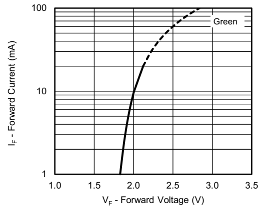
Fig. 18 - Forward Current vs. Forward Voltage
