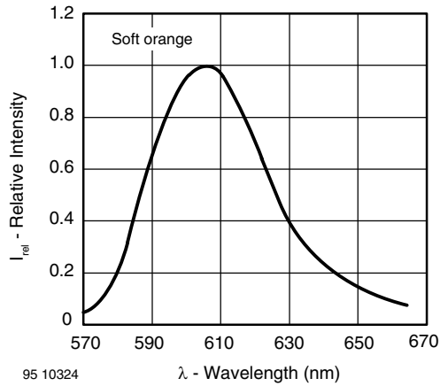
Fig. 8 - Relative Intensity vs. Wavelength
