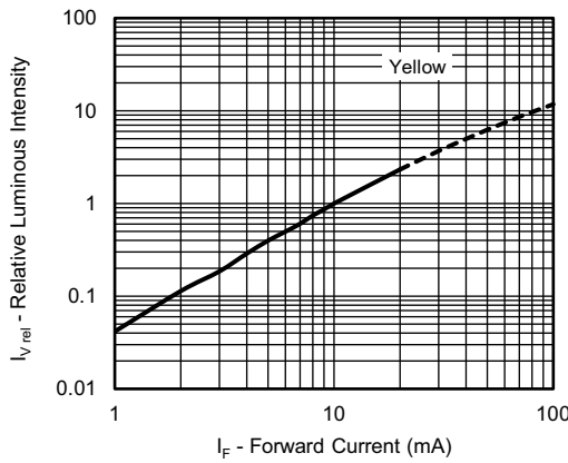
Fig. 14 - Relative Luminous Intensity vs. Forward Current
