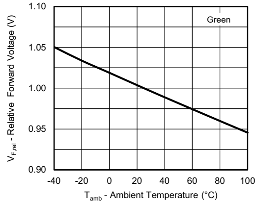
Fig. 21 - Relative Forward Voltage vs. Ambient Temperature
