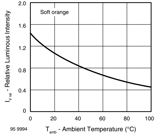
Fig. 11 - Relative Luminous Intensity vs. Ambient Temperature
