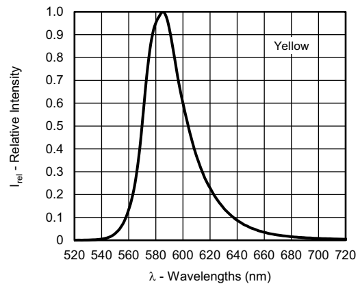
Fig. 12 - Relative Intensity vs. Wavelength
