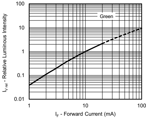
Fig. 19 - Relative Luminous Intensity vs. Forward Current
