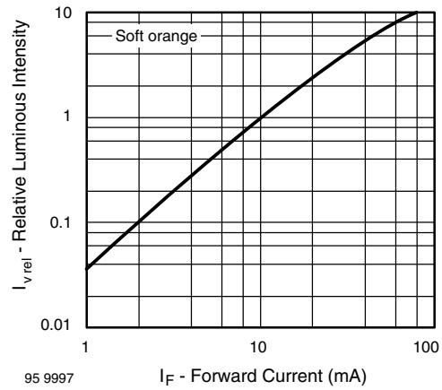
Fig. 10 - Relative Luminous Intensity vs. Forward Current
