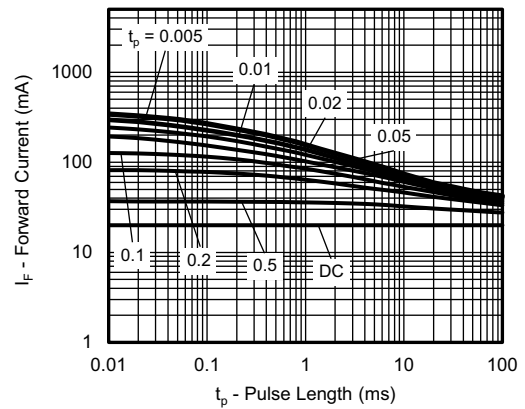
Fig. 22 - Permissible Pulse Forward Current vs. Pulse Duration
