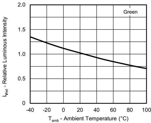
Fig. 20 - Relative Luminous Intensity vs. Ambient Temperature
