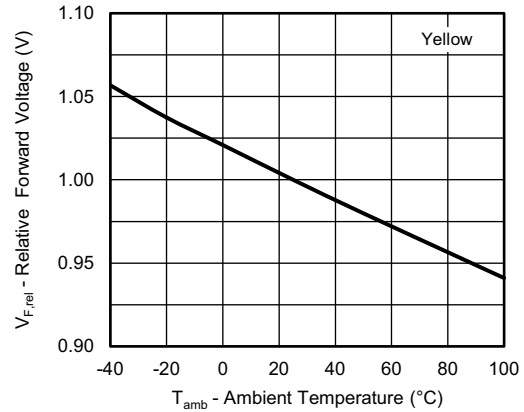
Fig. 16 - Relative Forward Voltage vs. Ambient Temperature
