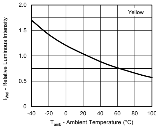
Fig. 15 - Relative Luminous Intensity vs Ambient Temperature
