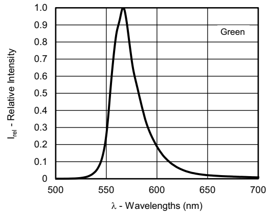
Fig. 17 - Relative Intensity vs. Wavelength
