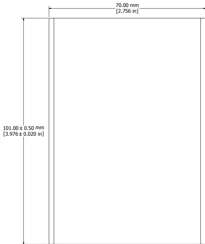
EXTRUSION
