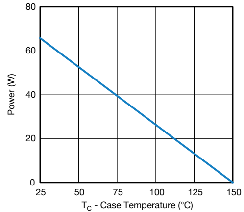
Power, Junction-to-Case
