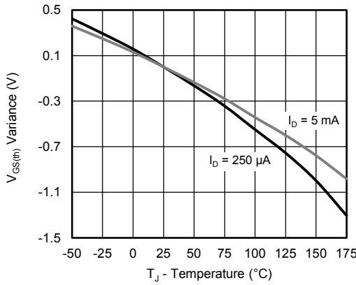
Threshold Voltage
