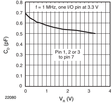
Fig. 4 - Typical Capacitance C D vs. Reverse Voltage V R
