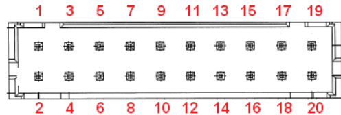
Signal Output Signal Connectors (SK2) SK2 Mating Connector: JST Part Number PHDR-20VS; Contact Pins: JST Part Number SPHD-001T-P0.5
