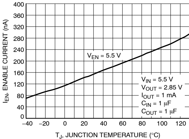
Figure 13. Current to Enable Pin vs. Temperature
