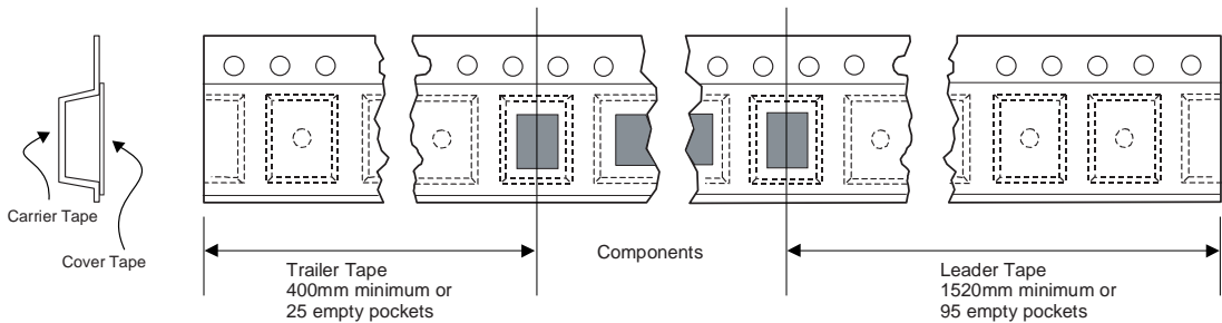
TO-263AB/D 2 PAK Tape Leader and Trailer Configuration: Figure 2.0
