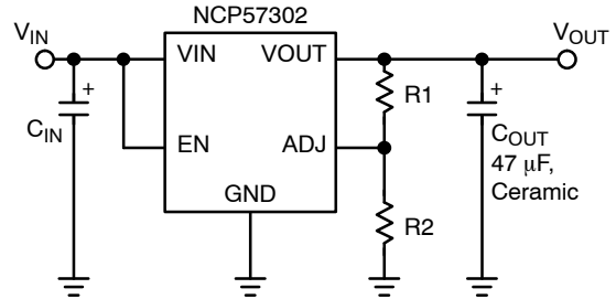
Figure 21. Adjustable Voltage Operation
