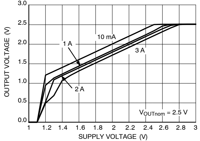
Figure 7. Dropout Characteristics
