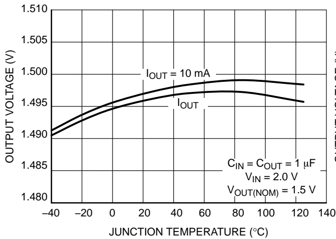
Figure 3. Output Voltage vs. Temperature V_{OUT} = 1.5\text{ V}
