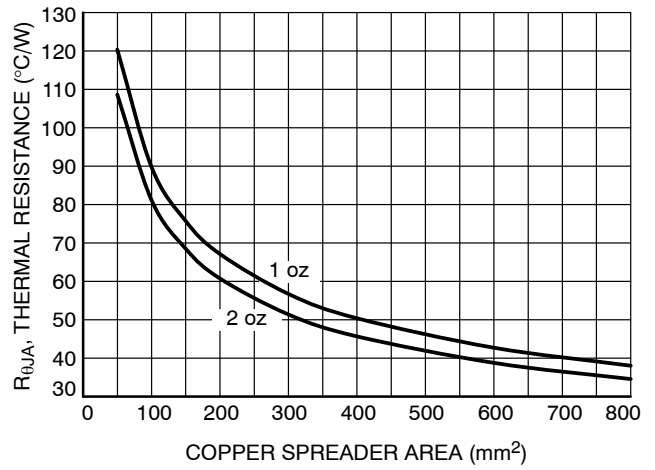
Figure 22. R θJA vs. Copper Spreader Area, D 2 PAK 3-Lead
