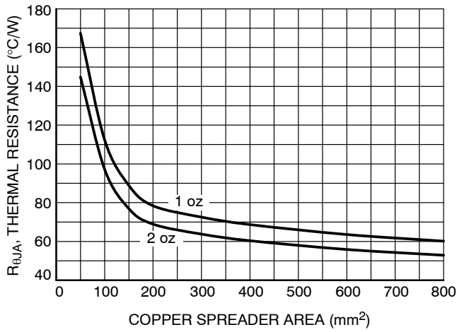
Figure 21. R θJA vs. Copper Spreader Area, DPAK 3-Lead
