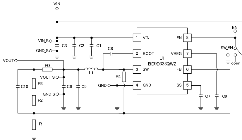
Figure 44. Application Circuit
