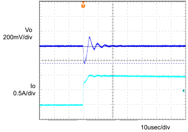
Fig.4 Transient Response (1.0→0A) Co=1µF, Ta=25°C
