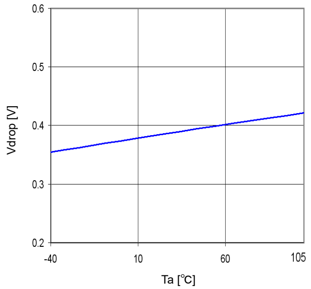
Fig.30 Minimum dropout Voltage1 ( V_{cc}=3.3\text{V} 、 I_o=1.0\text{A} )
