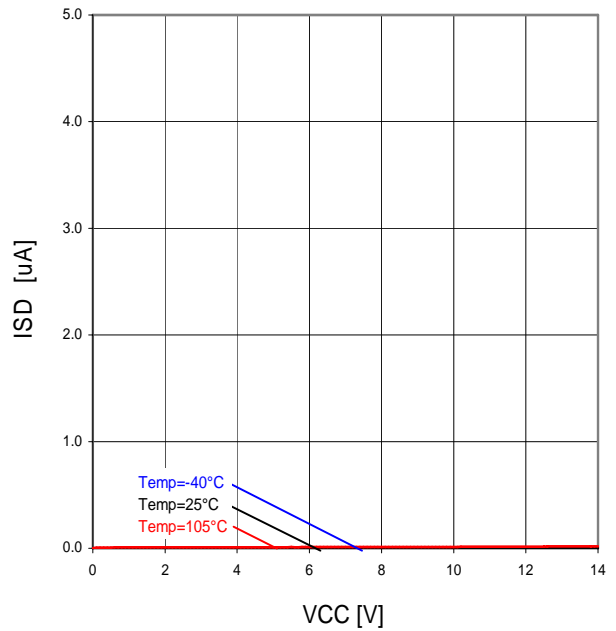
Figure 26. V_{CC}-I_{SD} ( V_{EN}=0V )
