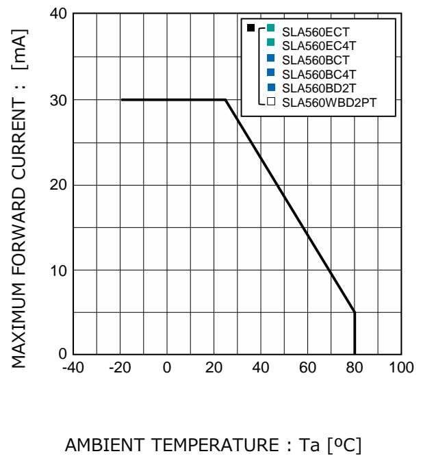
Fig.4 Derating
