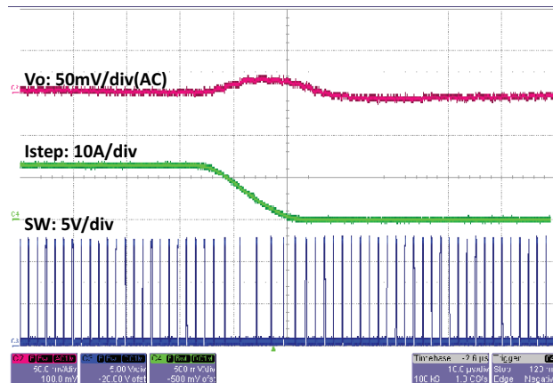
Fig. 37 - SiC451 Load Step, 12.5 A to 0 A, 1 A/ \mu\text{s} , t = 10\text{ }\mu\text{s/div}
