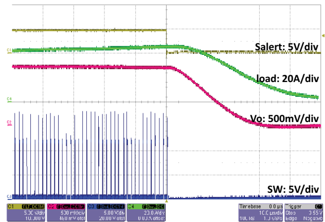
Fig. 49 - SiC450 Overcurrent Protection Behavior, t = 10\text{ }\mu\text{s}
