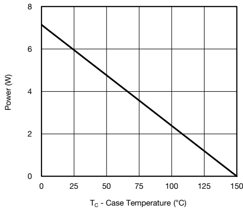
Power, Junction-to-Case
