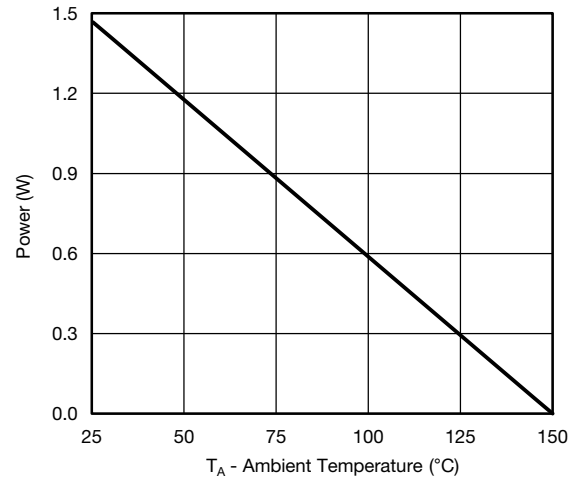
Power Derating
