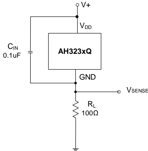
Low-side sensing
