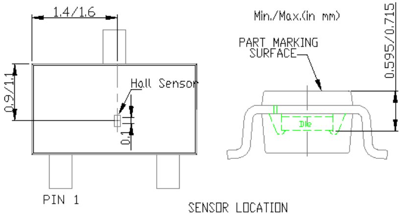
AH32xxQ Hall sensor
