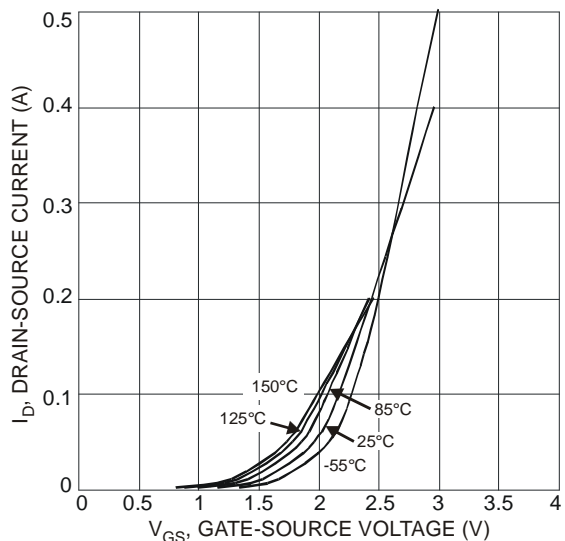
Fig. 10 Transfer Characteristics
