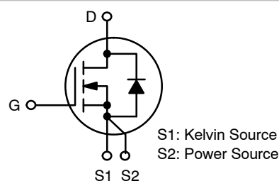
N-CHANNEL MOSFET
