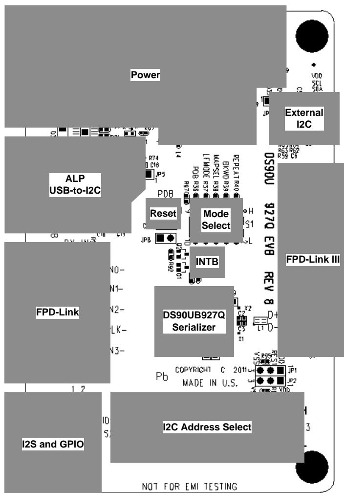
Figure 3-1. DS90UB927QEVMB Layout
