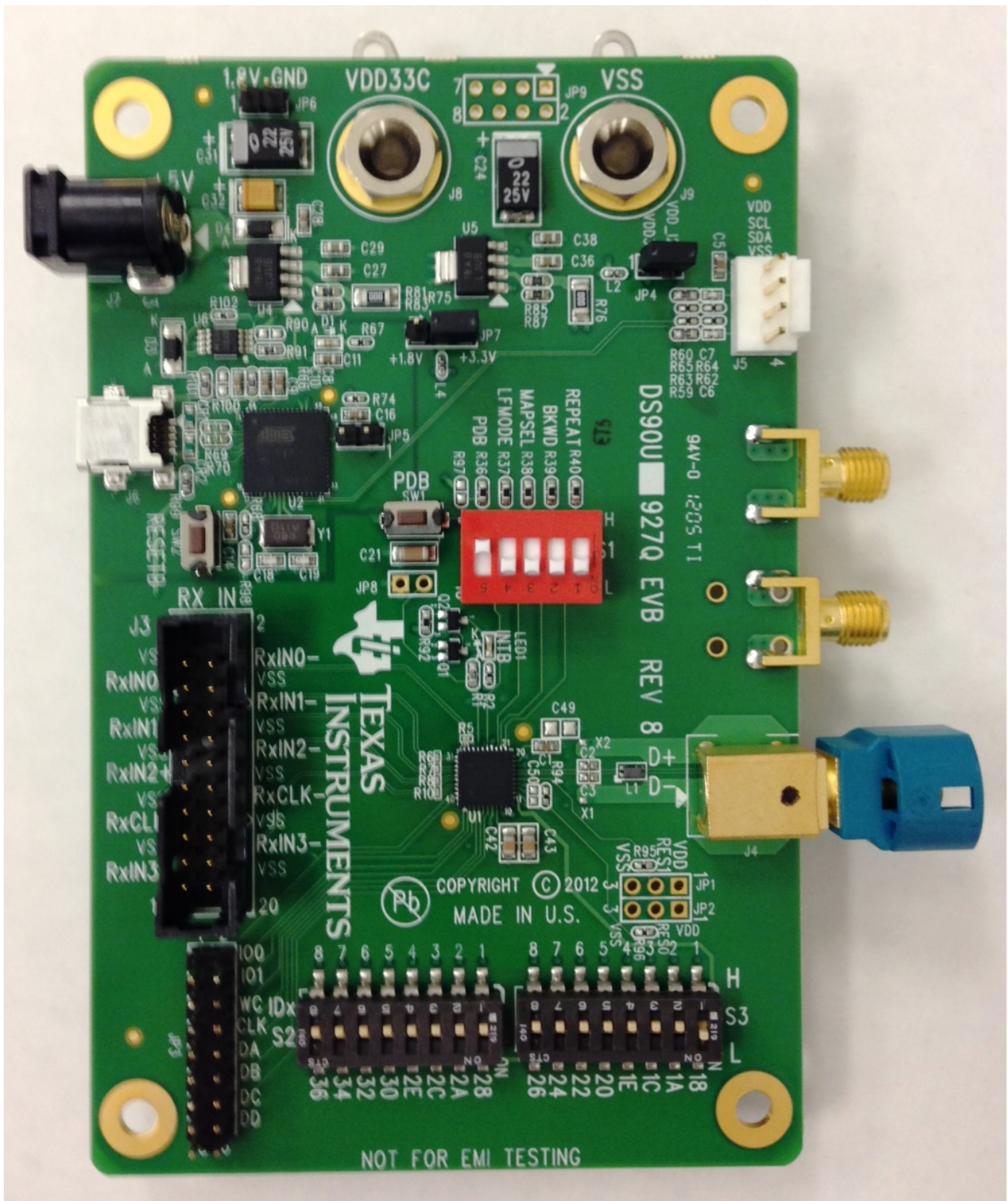
Figure 2-1. DS90UB927QEVM
