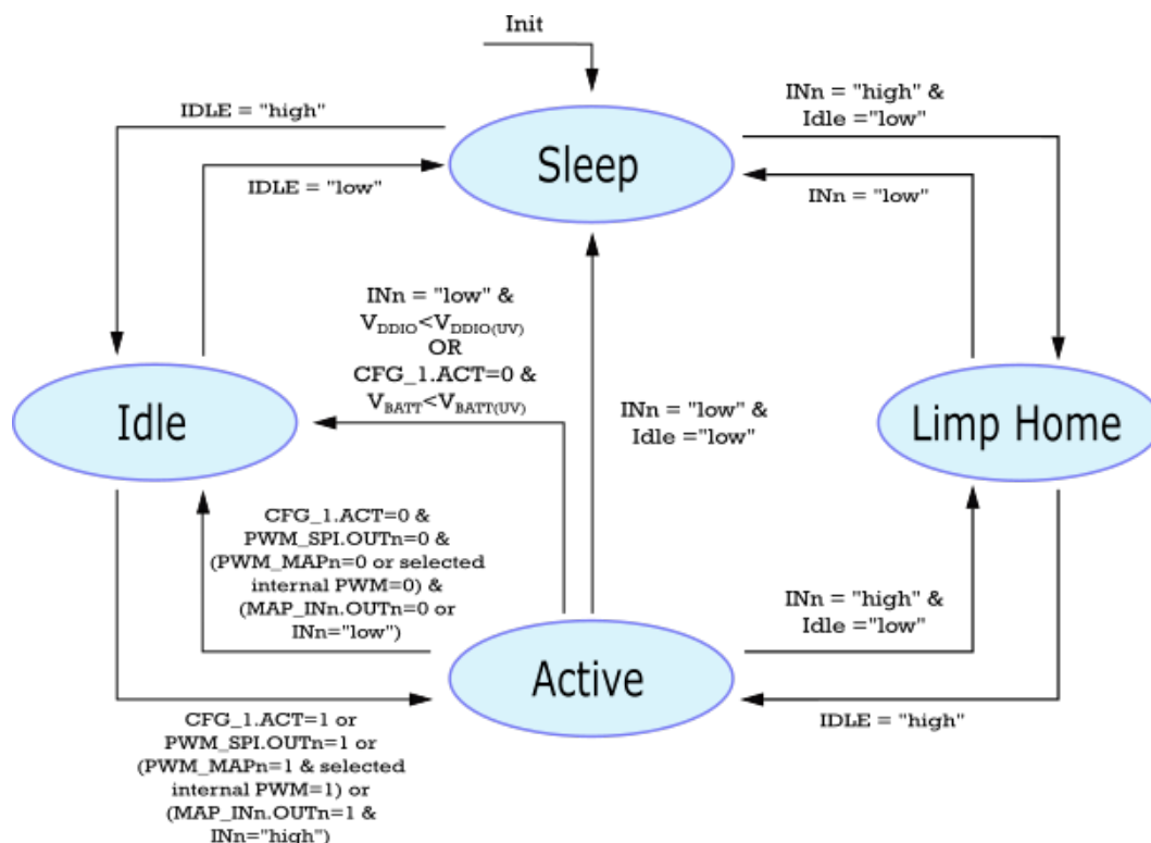
Figure 6. State diagram
