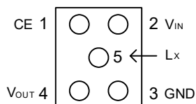
WLP-5-06 (BOTTOM VIEW)
