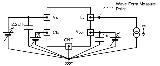
< Circuit No.⑥ >
