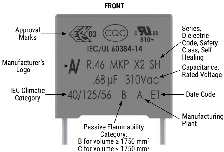
Manufacturing Date Code (IEC-60062)
