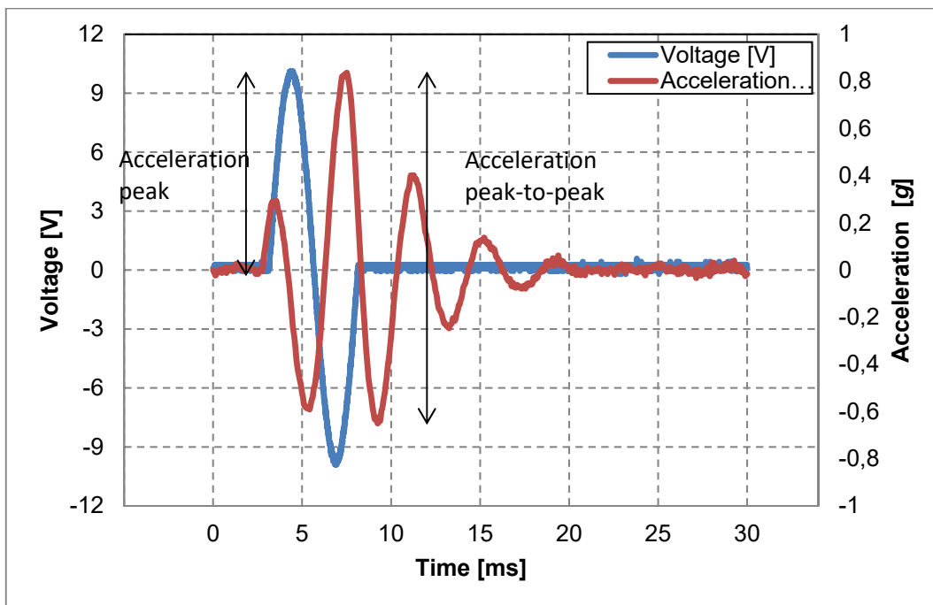
Fig. 6: Typical acceleration g as a function of input voltage with 100 g load. Input voltage with a sinus signal form of amplitude -10 \dots 10 V and pulse length 5 ms which is equivalent to 200 Hz.
