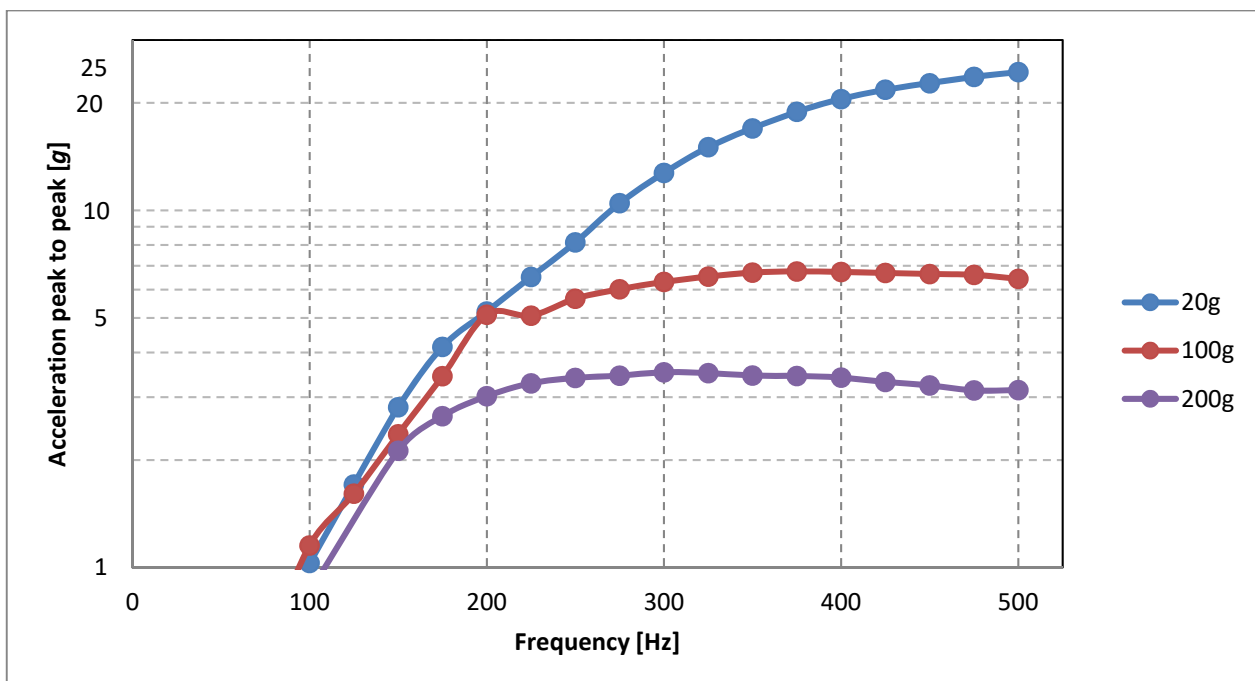
Fig. 7: Acceleration g as a function of frequency for different loads. Input voltage has a single pulse half wave sinus signal form of amplitude 0 \dots 60 V and varying frequency from 50 ... 500 Hz.
