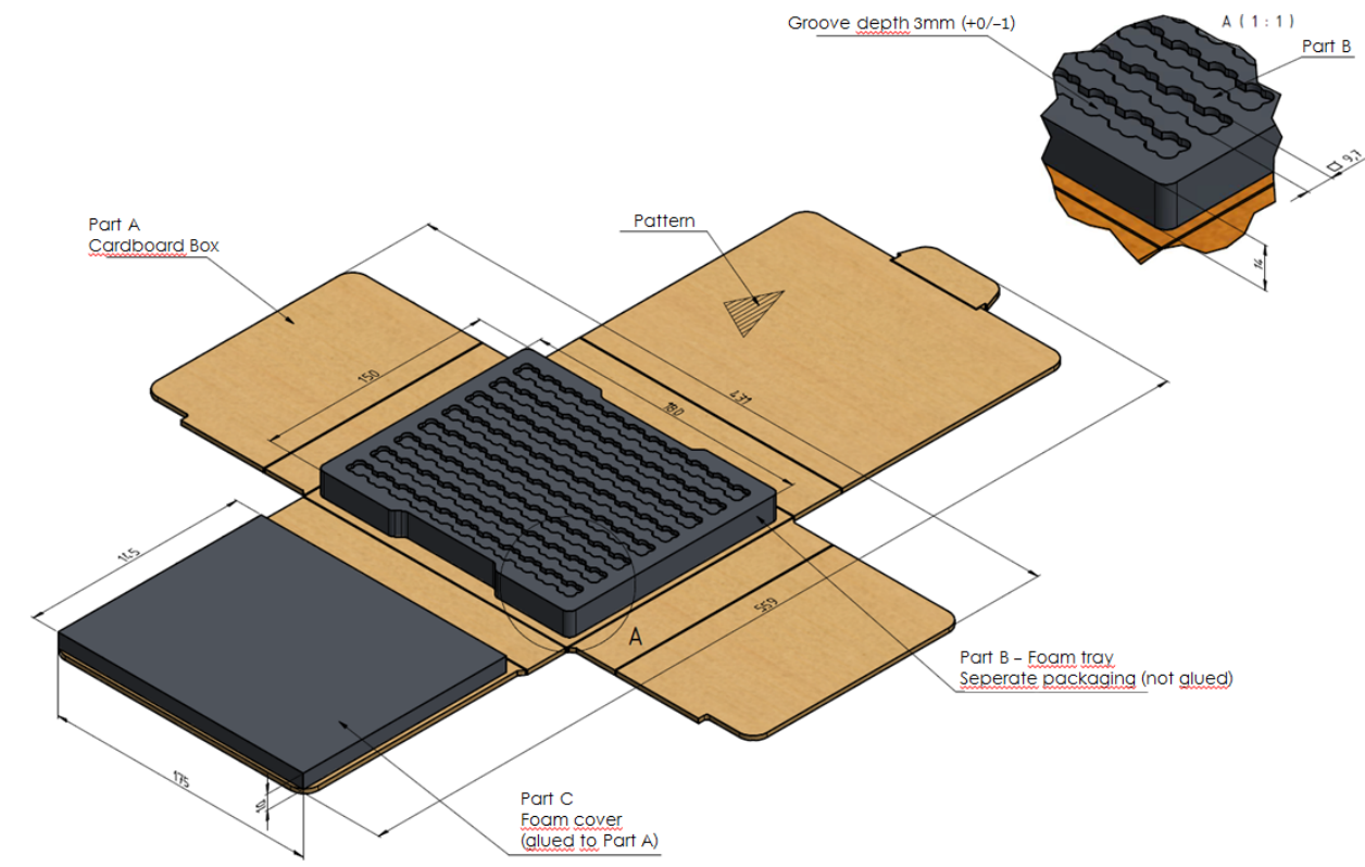
Fig. 18: Drawing of the packaging unit.
