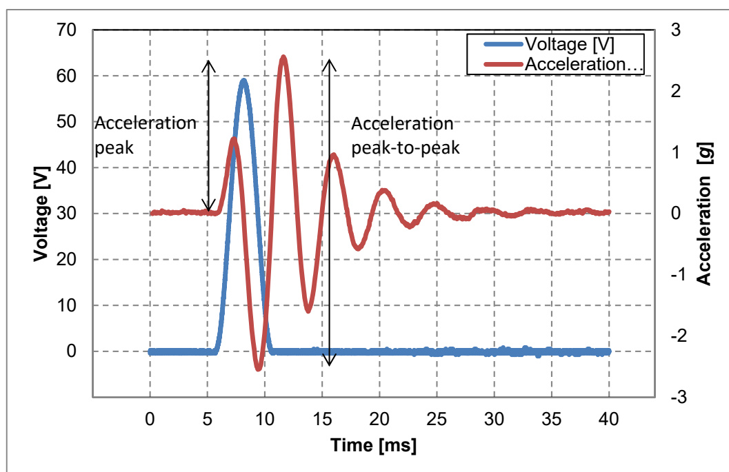
Fig. 5: Typical acceleration g as a function of input voltage with 100 g load. Input voltage with a half wave sinus signal form of amplitude 0 ... 60 V and pulse length 5 ms which is equivalent to 200 Hz.
