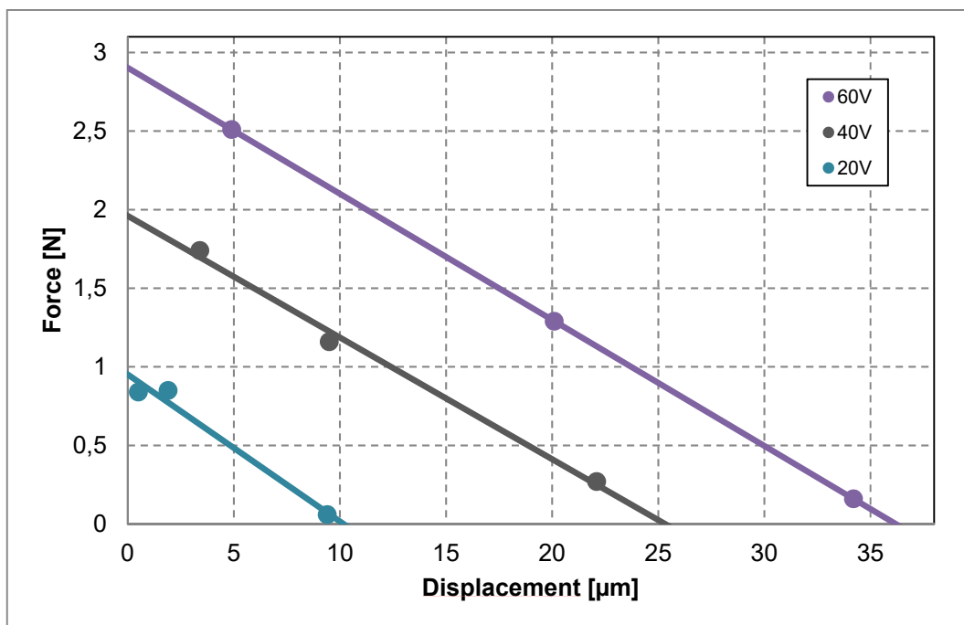
Fig. 3: Force-stroke diagram with different load springs. Typical stiffness 80 N/mm.
