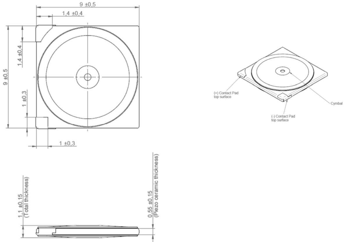
Fig. 1: Dimensional drawings
