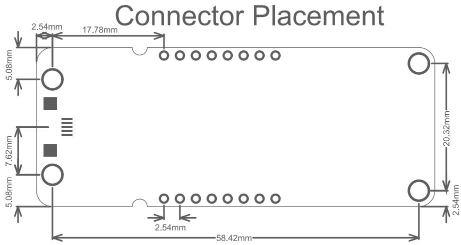
Figure 7-4. Connector Placement
