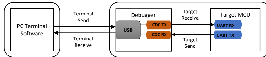
Figure 4-1. CDC Connection
