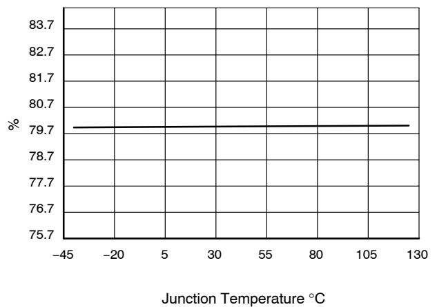
D_{MAX1a(200 kHz)}
