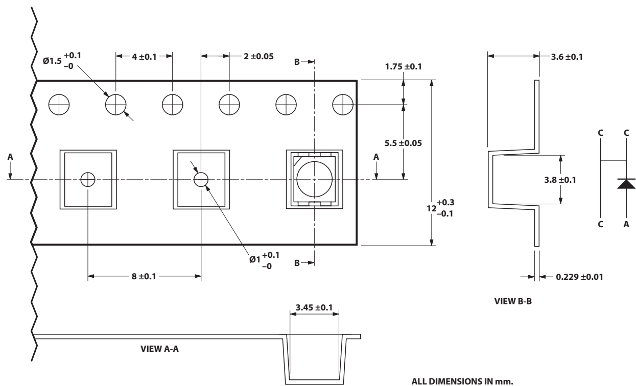
Figure 14: Tape Dimensions
