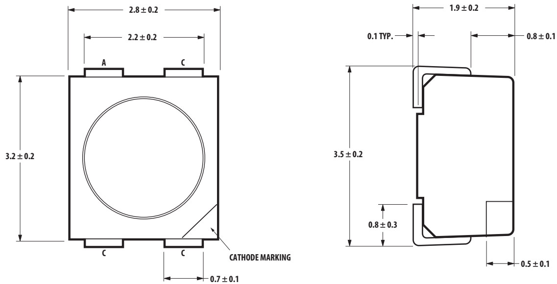
Figure 1: Package Dimensions
