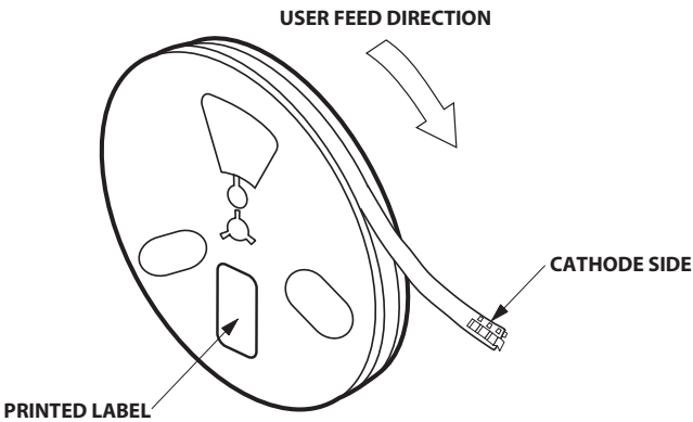
Figure 15: Reeling Orientation
