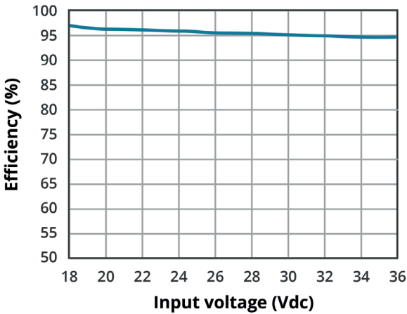
EFFICIENCY VS INPUT LOAD P7815-2000-S (full load)
