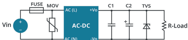
Fig. 1: Typical circuit diagram
