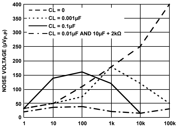
FIGURE 43. NOISE REDUCTION
