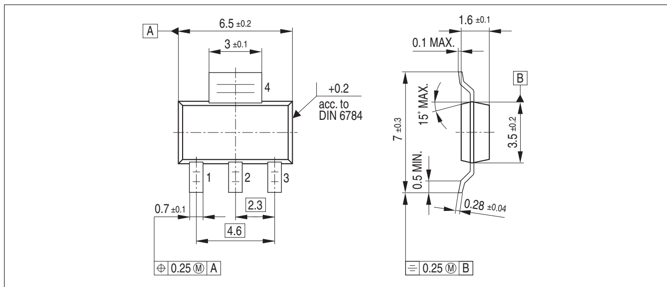
Figure 5 PG-SOT223-4 1)
