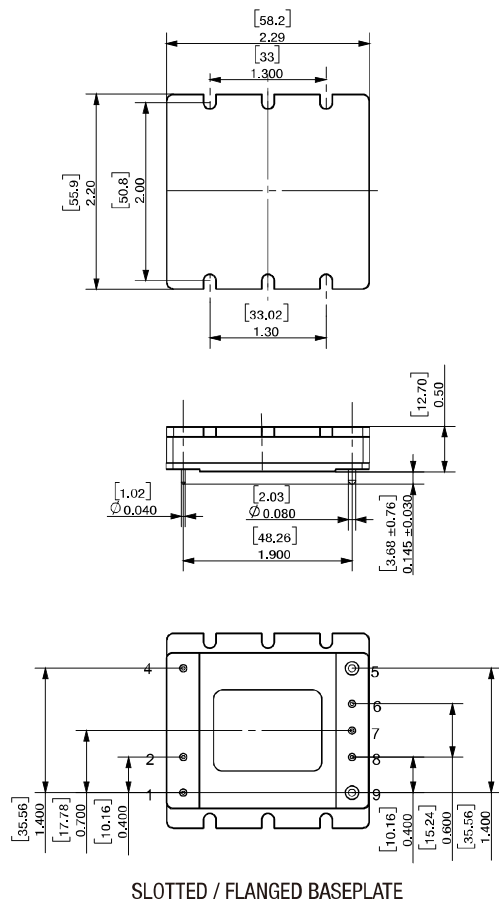
Slotted / Flanged Baseplate
