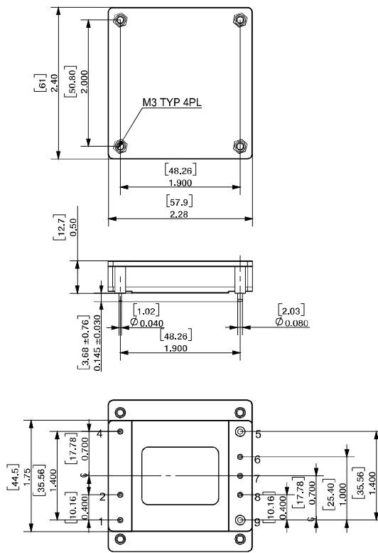
Standard Baseplate
