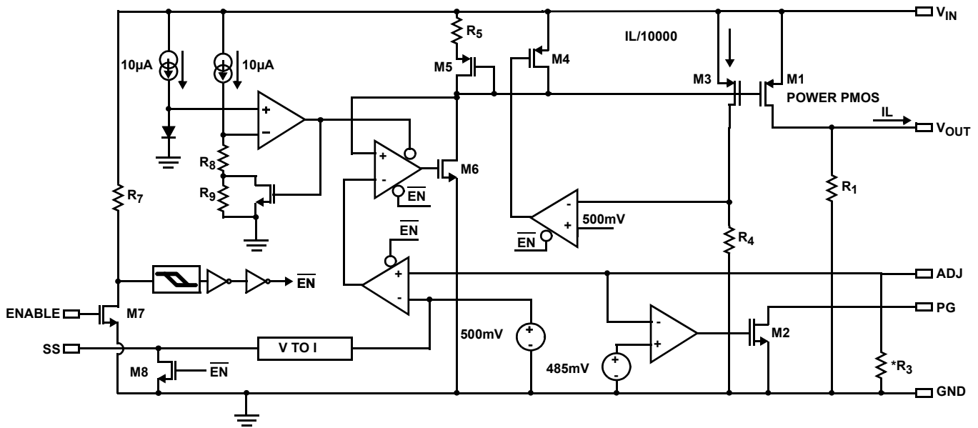
FIGURE 2. BLOCK DIAGRAM
