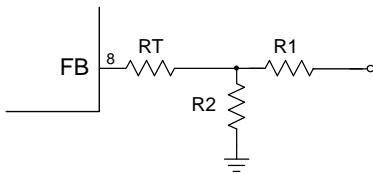
Figure 4: T-Type Network
