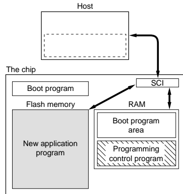
Figure 22.4 Boot Mode
