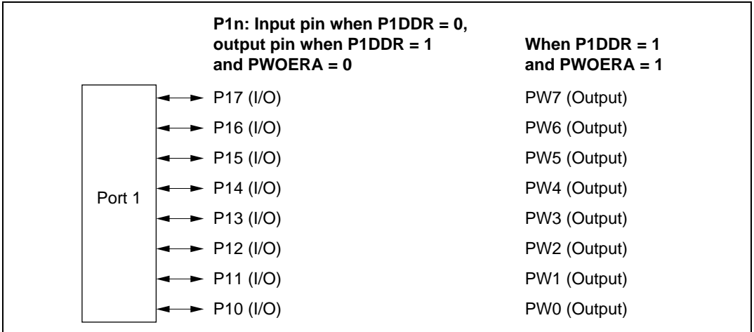
Figure 8.4 Port 1 Pin Functions (Modes 2 and 3 (EXPE = 0))
