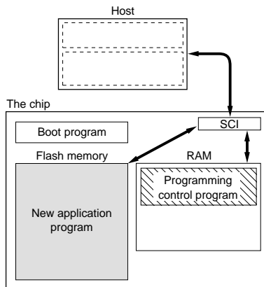
Figure 21.4 Boot Mode
