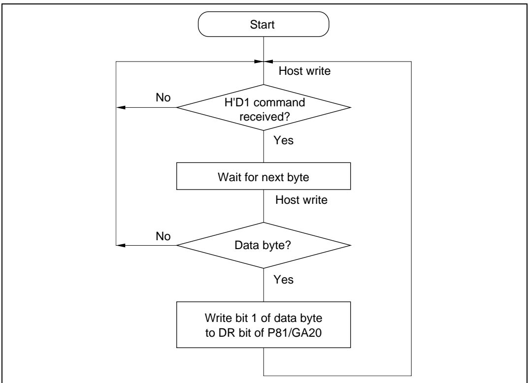
Figure 17.2 GA20 Output
