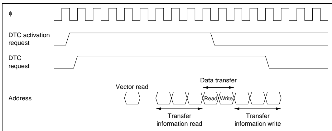
Figure 7.10 DTC Operation Timing (Normal Mode or Repeat Mode)
