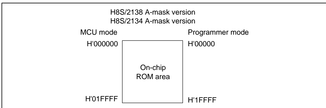
Figure 22.15 Memory Map in Programmer Mode
