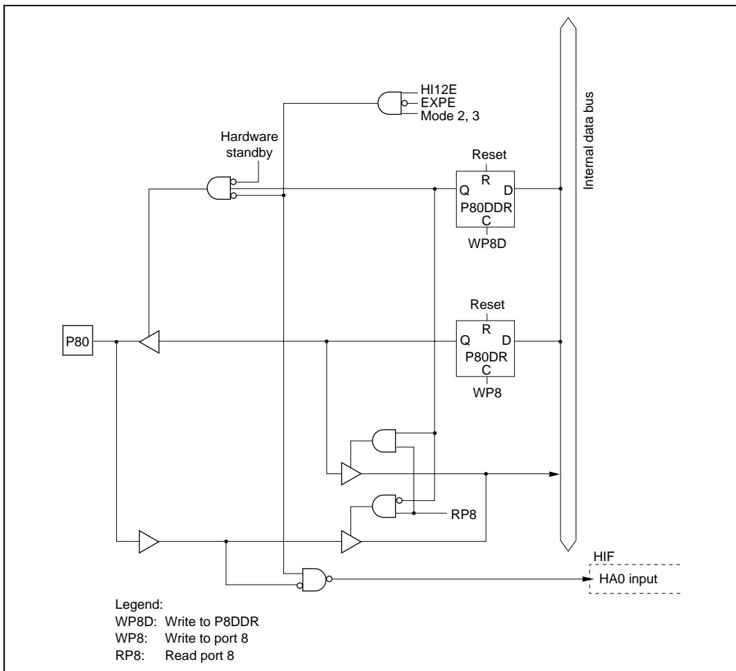
Figure C.23 Port 8 Block Diagram (Pin P80)
