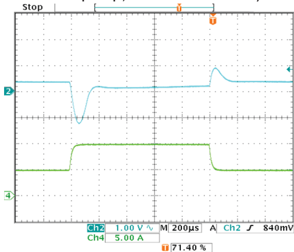
Stepload Transient Response (Vin=48V, Iout=50-75-50% of Iout, Cload= 1μF || 10μF || 4700μF, Slew rate: 5A/uS at Ta=+25°C)
