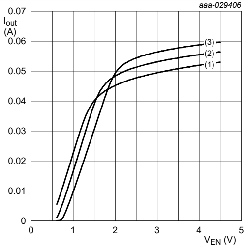
V_{out} = 2\text{ V} ; R_{ext} = 20\ \Omega (1) R_{ext} = 85\text{ }^\circ\text{C} (2) R_{ext} = 25\text{ }^\circ\text{C} (3) R_{ext} = -40\text{ }^\circ\text{C}
