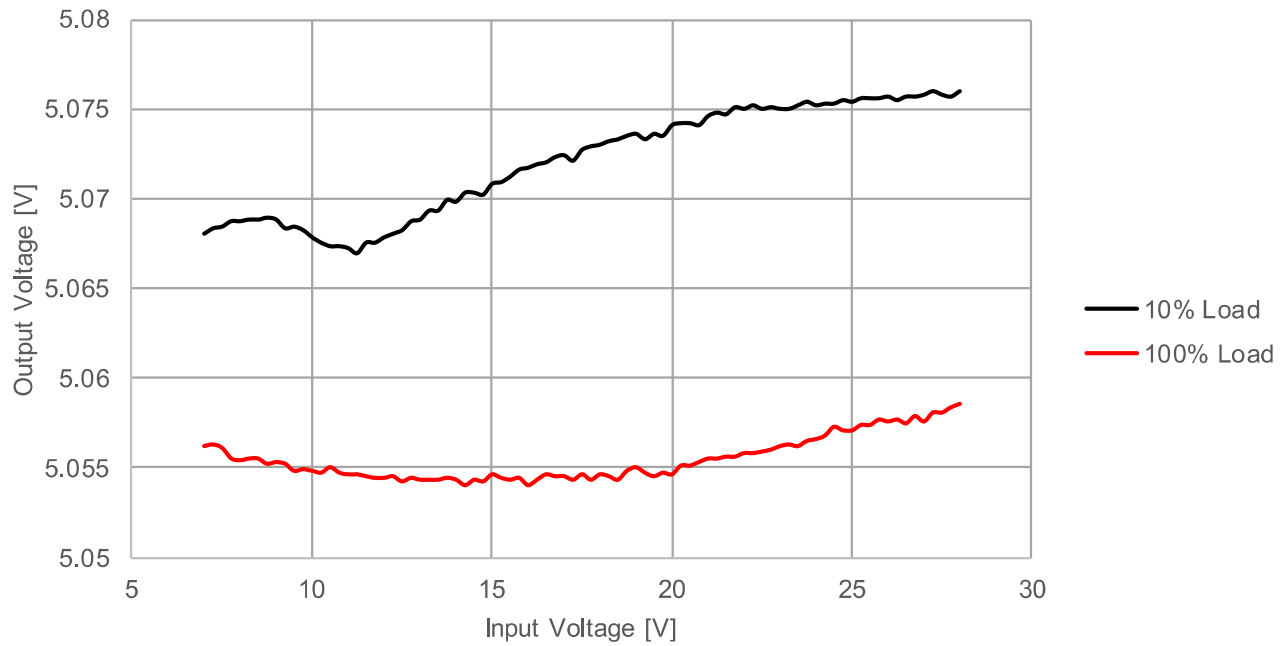
173950578 Line Regulation V_{OUT} = 5V , T_A = 25^\circ C
