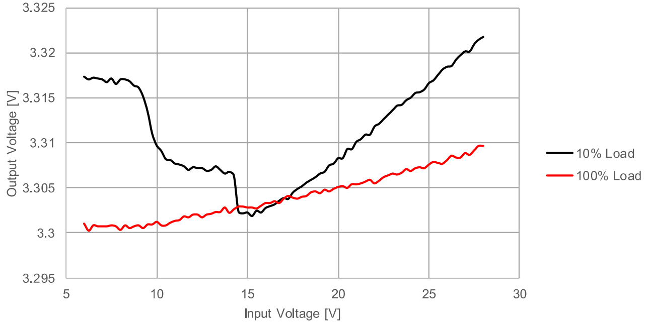
173950378 Line Regulation V_{OUT} = 3.3V , T_A = 25^\circ C
