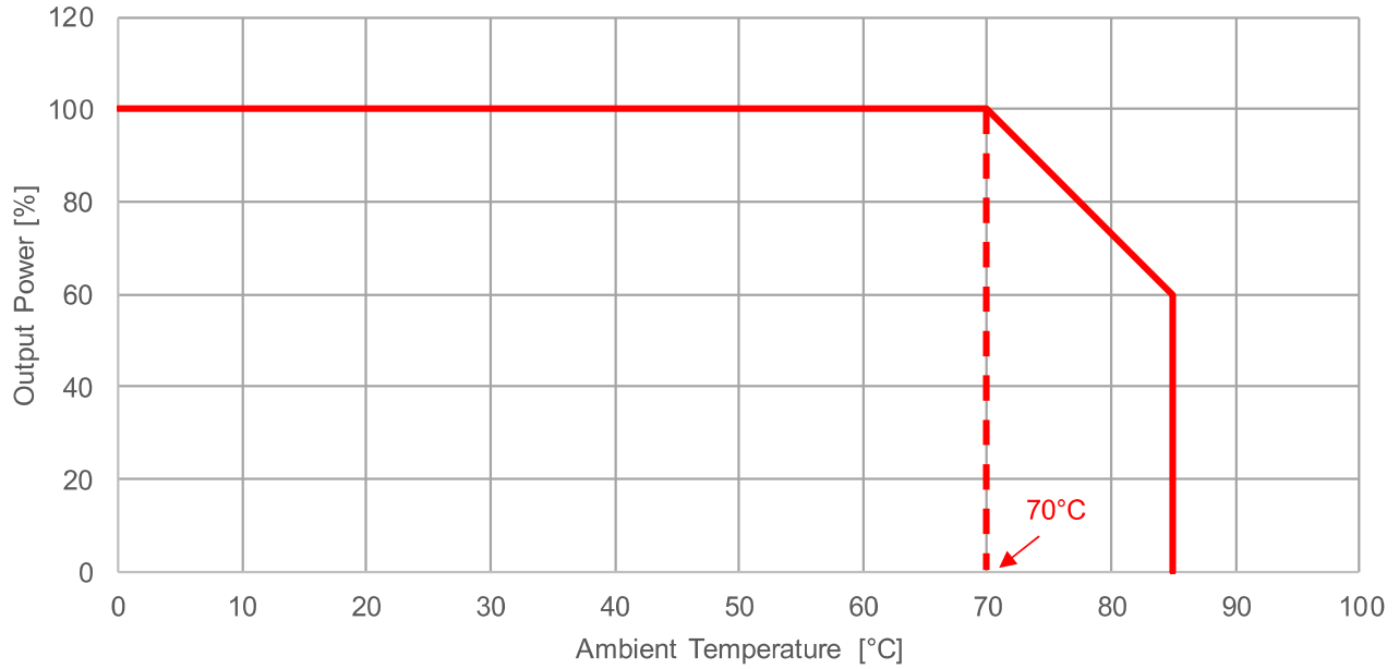
173950x78 Output Power Thermal Derating V_{IN} = 24V , I_{OUT} = 500mA & f_{SW} = 570kHz
