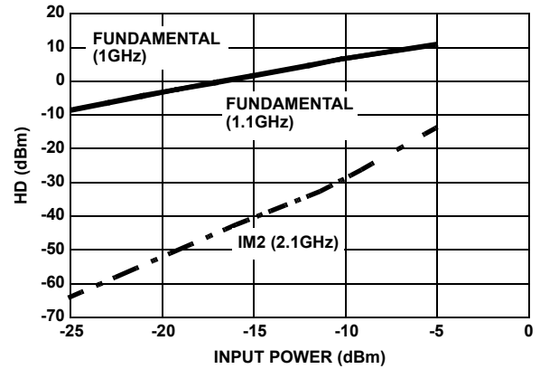
FIGURE 10. IM2 vs INPUT POWER
