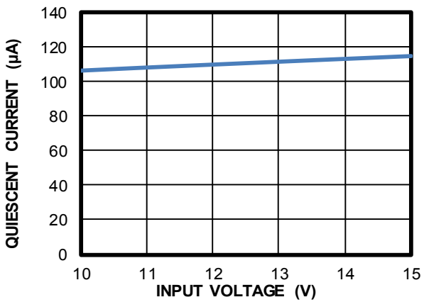
Quiescent Current vs. Input Voltage (12V E-Fuse)
