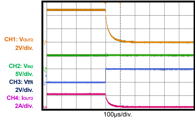
Current Limit (5V E-Fuse)
