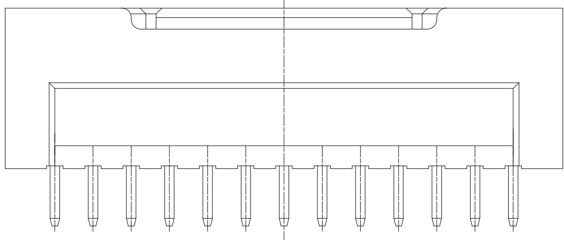
ENGAGEMENT FIGURE (2:1)
