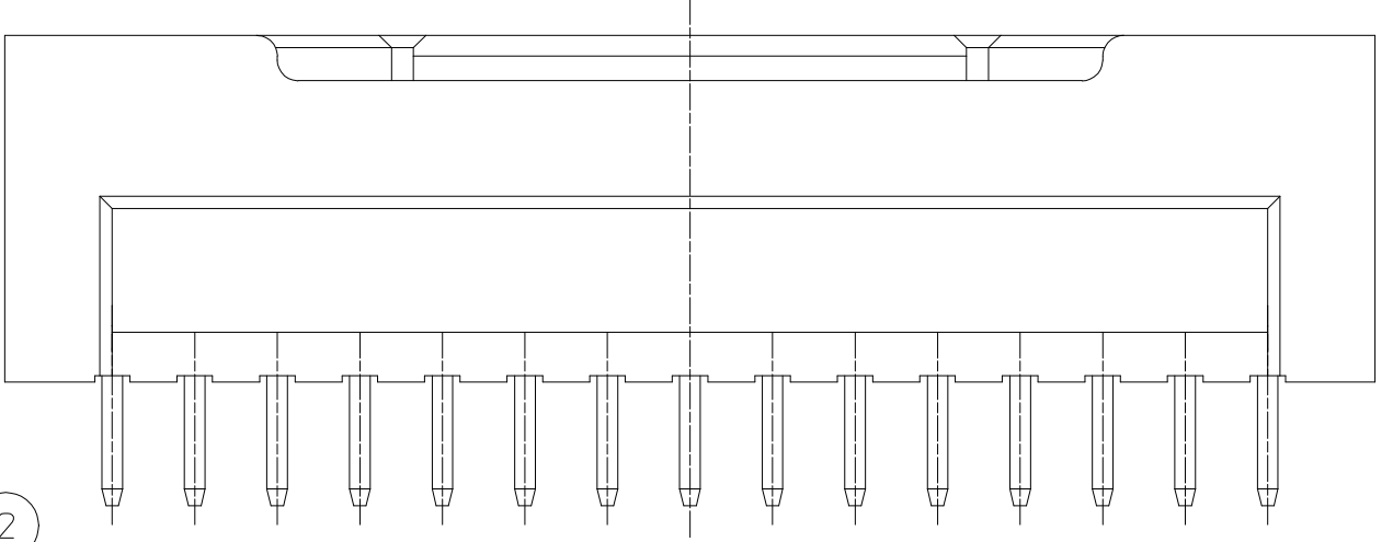
ENGAGEMENT FIGURE (2:1)
