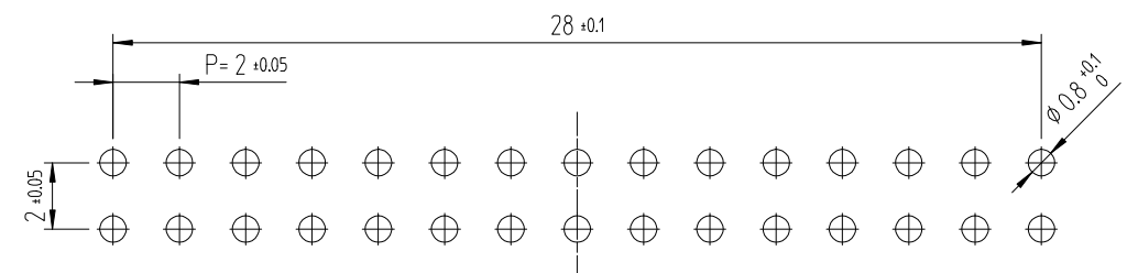
RECOMMENDED LAND PATTERN (FREE) (PCB THICKNESS t=1.6mm)
